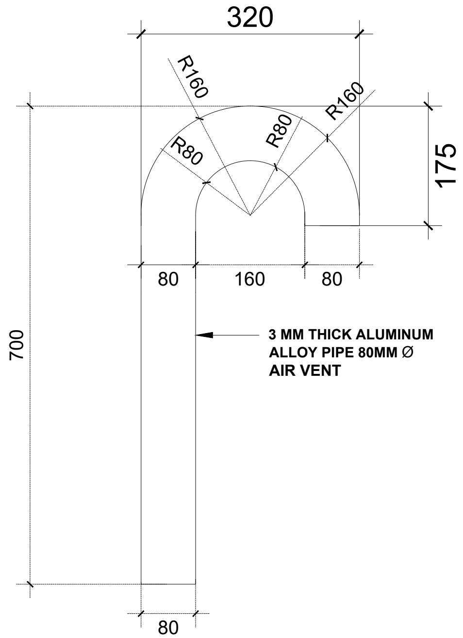
AIR VENT PIPE SIDE VIEW SCALE 1:3
