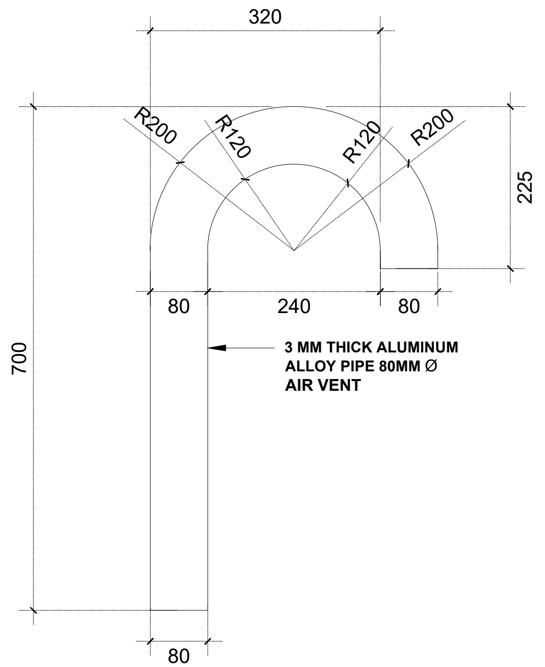
AIR VENT PIPE SIDE VIEW SCALE 1:3
